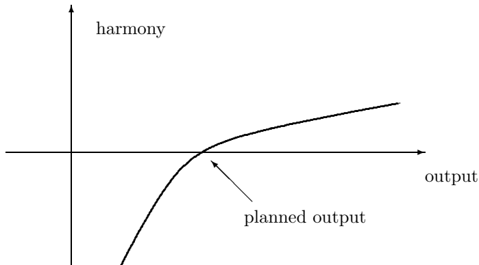
Figure 6.4: Harmony function
